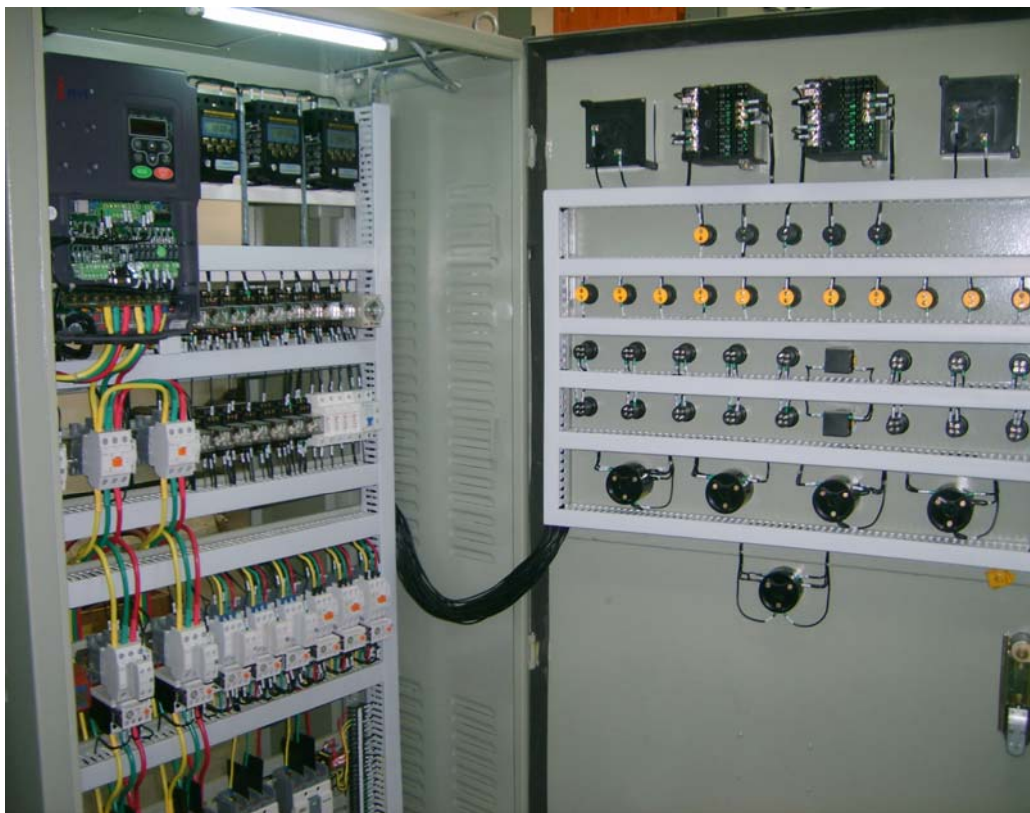
Wiring in Automatic Constant Pressure Water Supply Cabinet (2)
